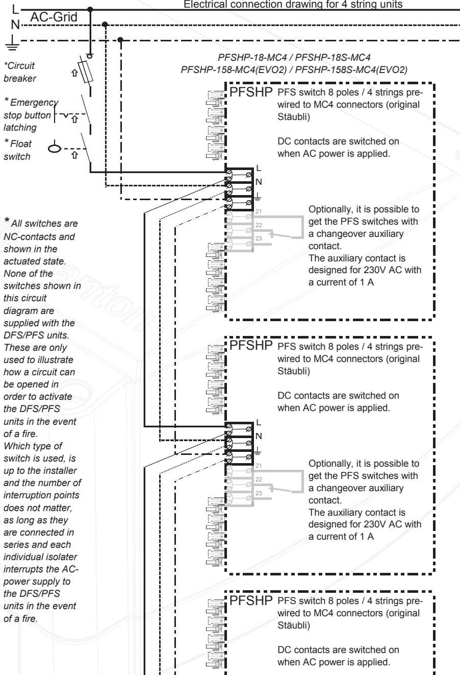
Electrical connection drawing for 4 string units
